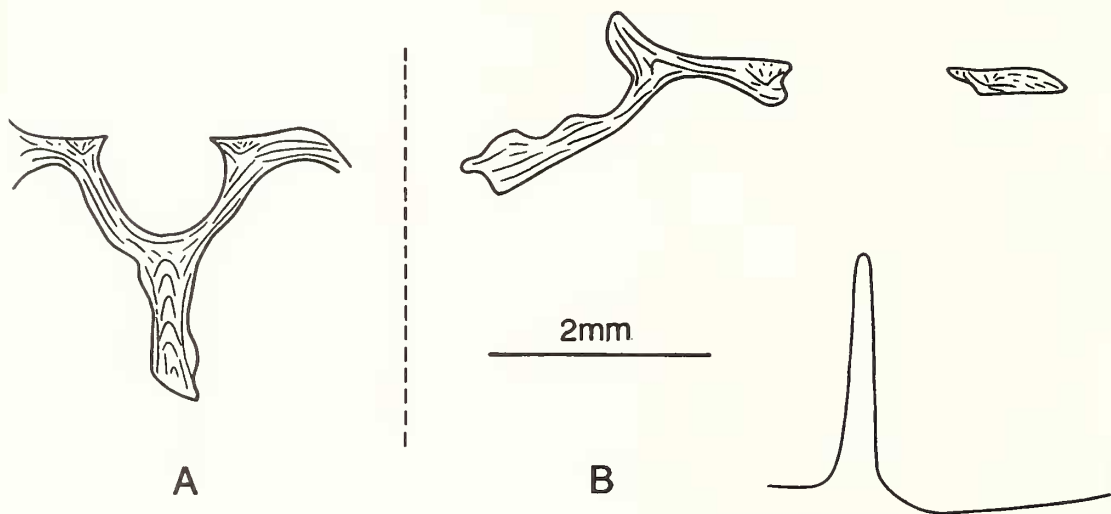
TEXT-FIG. 10. Transverse peels of Y. hanburyi Morphotype 1, showing broad septalium (A) and the absence of connectivum (B). Sample T12, a biplicate specimen (PUM92058).
